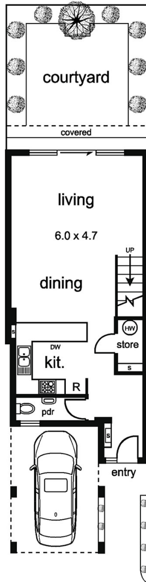
GROUND FLOOR
